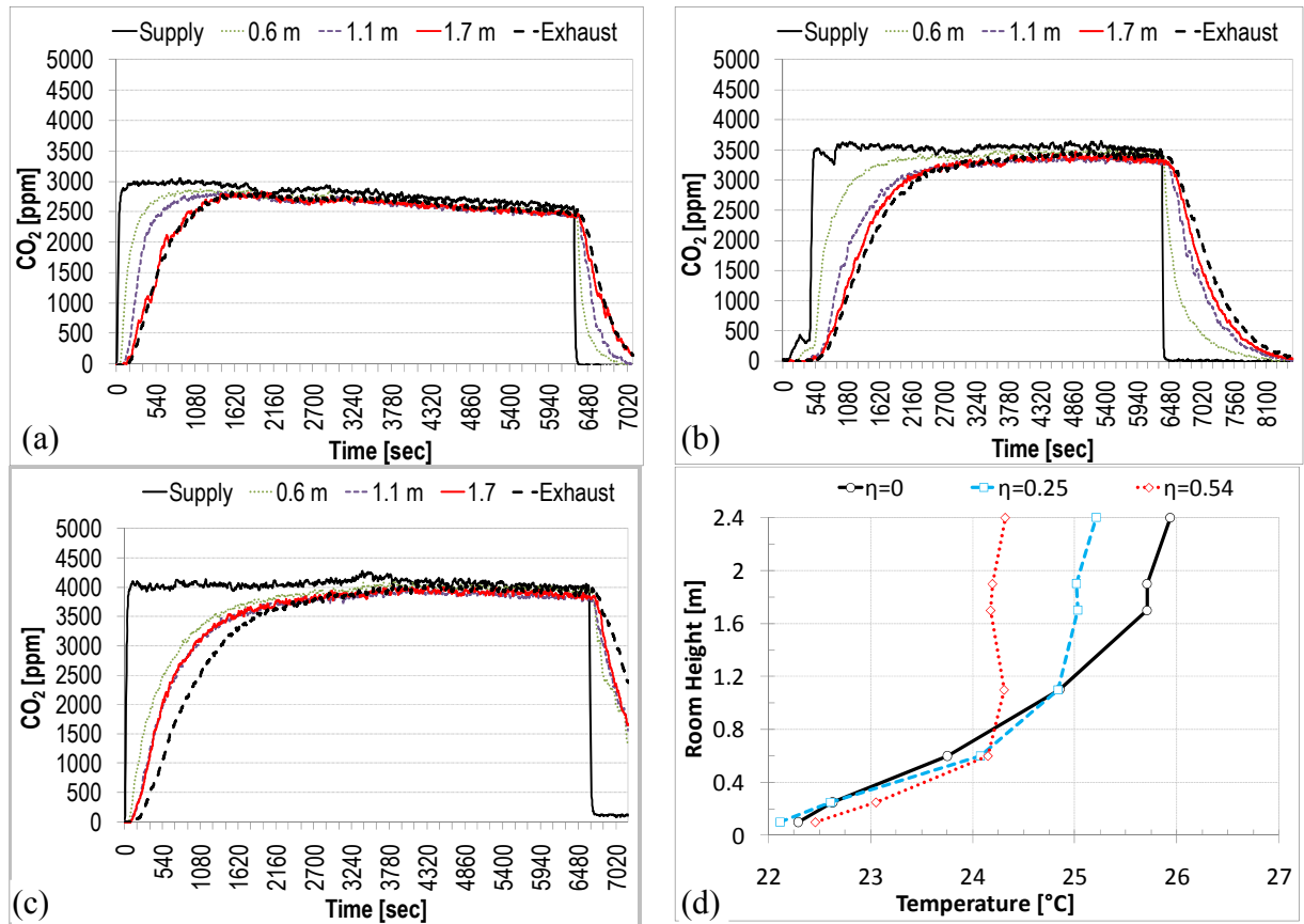
Figure 3. For (a) (b) and (c): CO 2 concentrations for the step-up method at the supply, exhaust and at 0.6, 1.1 and 1.7 m for: (a) test 1 where there is only DV; (b) test 2 where the radiant panels remove 25% of the load; and (c) test 3 where the radiant panels removed 54% of the load. (d) Air temperature profiles for the three tests described in Table 2.
