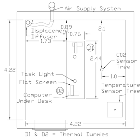
Figure 2. Layout of test chamber.
