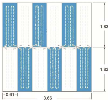
Figure 1. Active radiant panels (blue) configuration.
