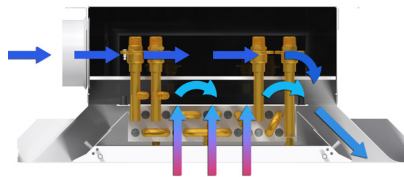
1-Way airflow
